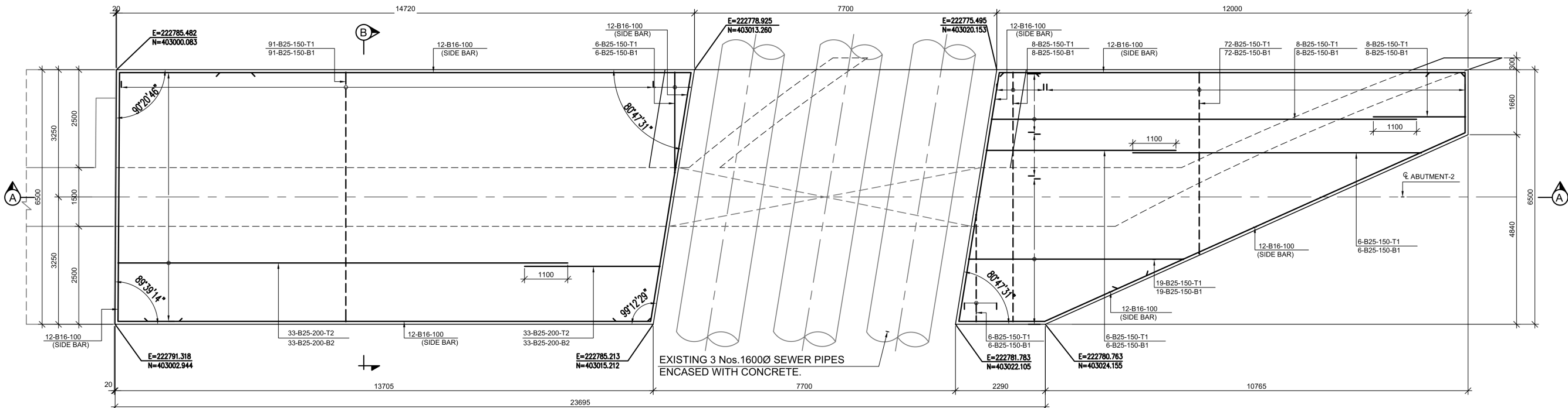
SECTION C-C SCALE: 1/50 TYPICAL LAP LENGTH Bar Size Lap Length (min.) Bar Size B16-150 800 B16 B16-125 1120 B16 B20-150 950 B20 B20-125 1330 B20
