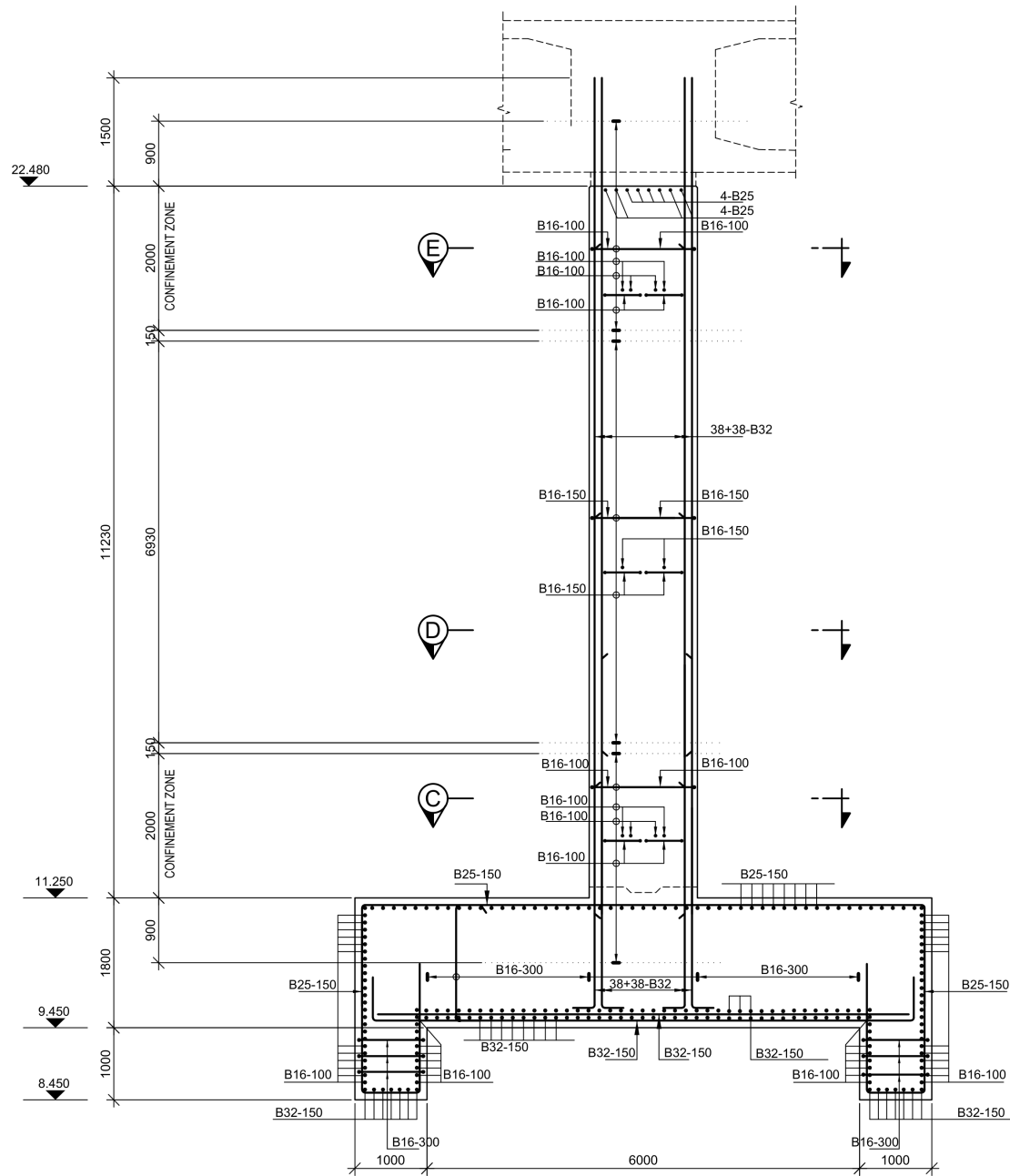
SECTION B-B SCALE:1/50
