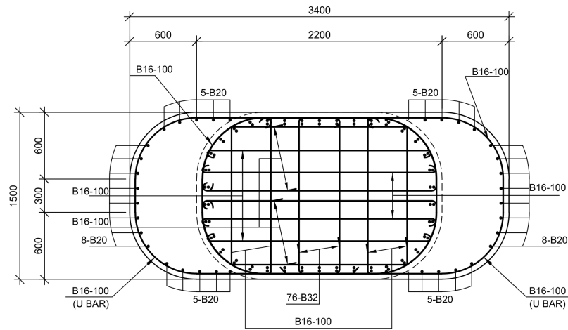
SECTION E-E SCALE:1/25
