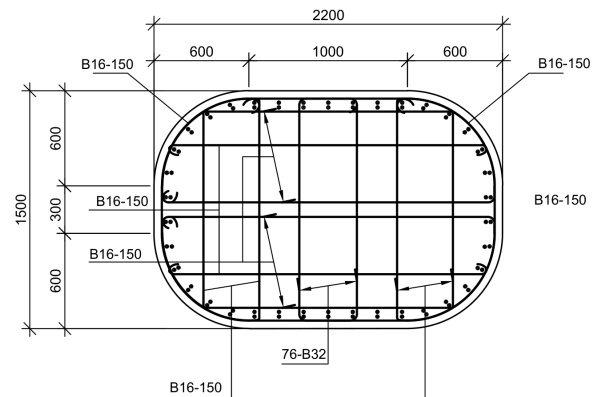
SECTION D-D SCALE:1/25
