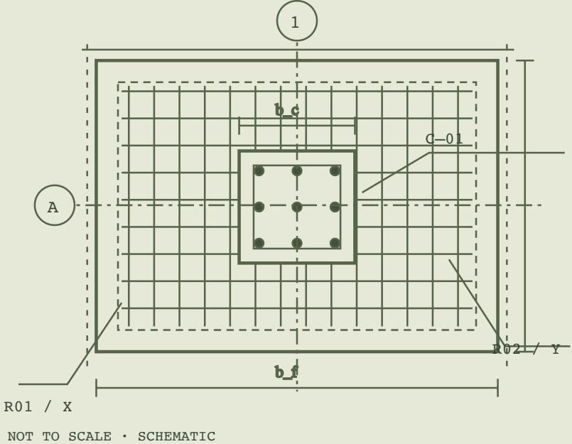
01 / FOUNDATION PLAN
