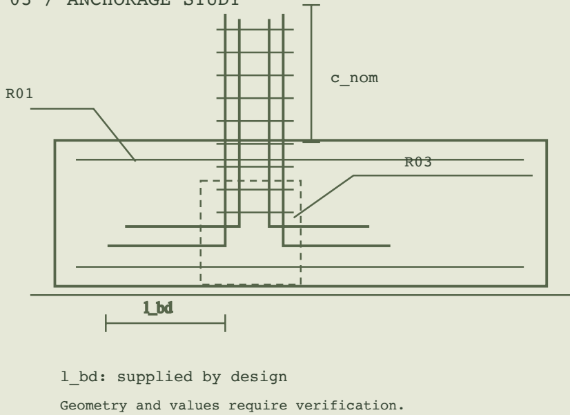
03 / ANCHORAGE STUDY
